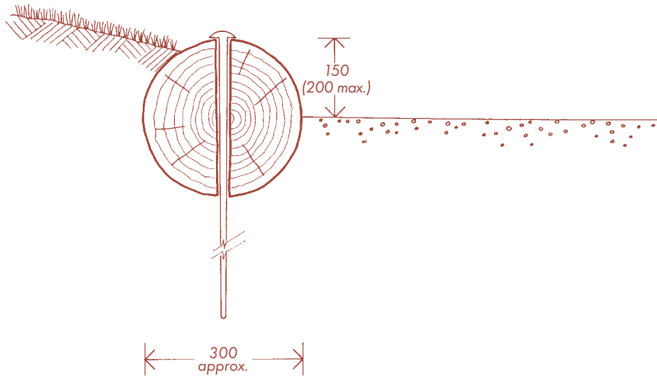
1.4A Section Scale 1:10 0 500mm
