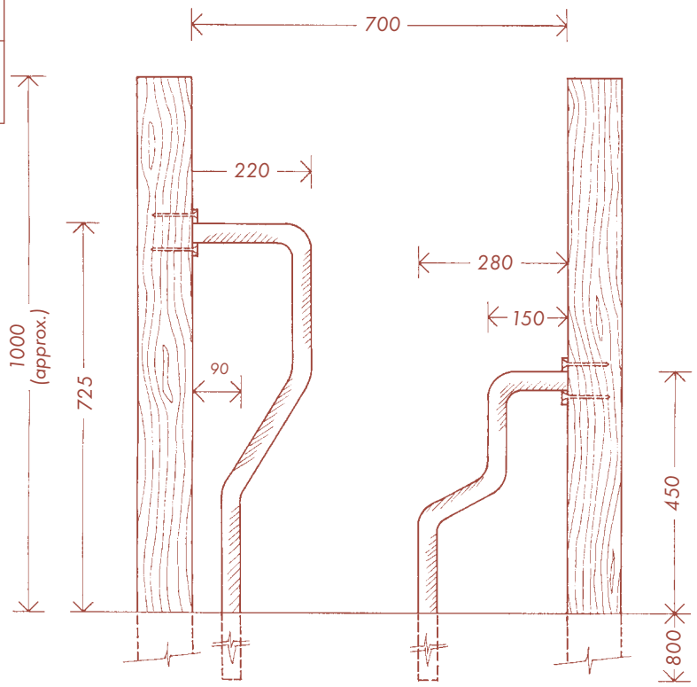
1.6B Fife Chicane : Front Elevation Scale 1:12.5 0 100mm
