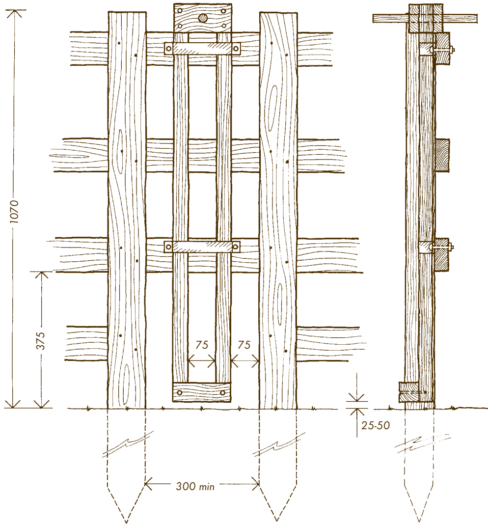
3.11A Elevation Scale 1:10 0 500mm
