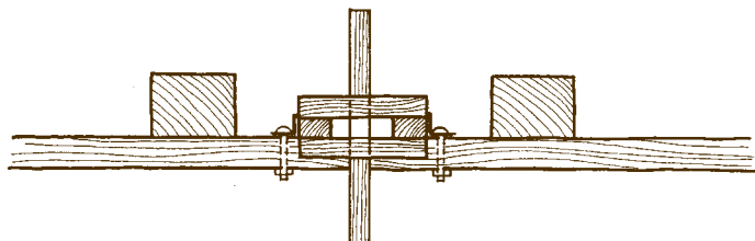
3.11C Plan Scale 1:10 0 500mm
