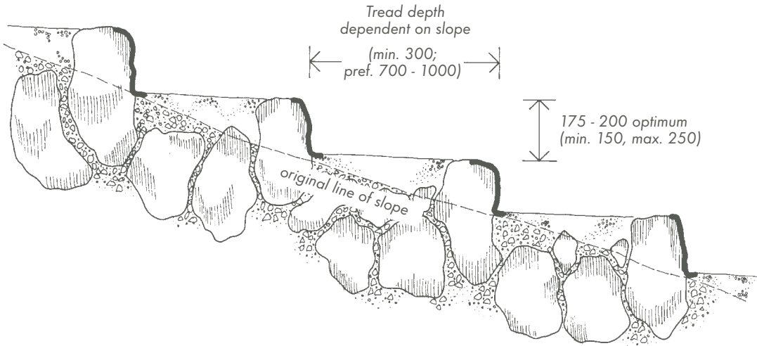
4.3A Section Scale 1:20 0 1000mm
