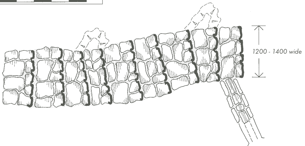
4.4B Plan Scale 1:50 0 2000mm
