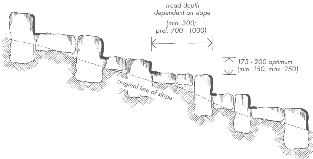
4.4A Side Elevation Scale 1:20 0 1000mm
