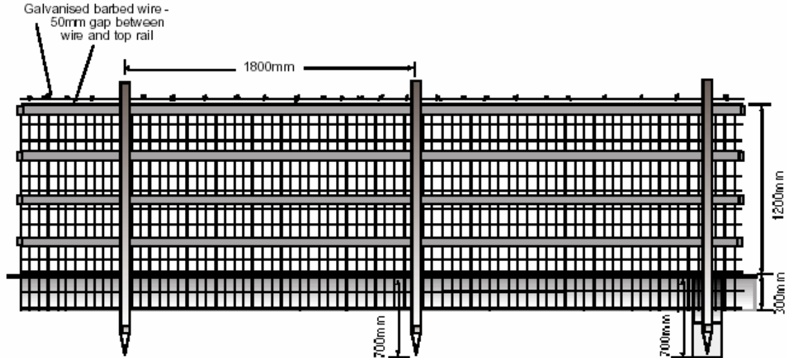
OTTER RESISTANT MESH ATTACHED TO A TIMBER & FOUR RAIL FENCE
